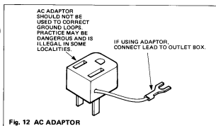
Fig. 12 AC ADAPTOR
