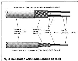
Fig. 8 BALANCED AND UNBALANCED CABLES
