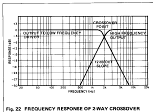
Fig. 22 FREQUENCY RESPONSE OF 2-WAY CROSSOVER
