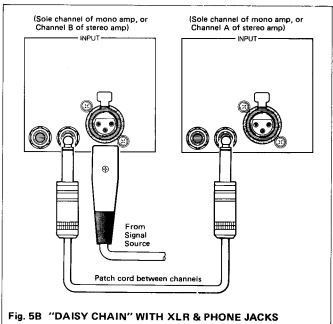
Fig. 5B "DAISY CHAIN" WITH XLR & PHONE JACKS
