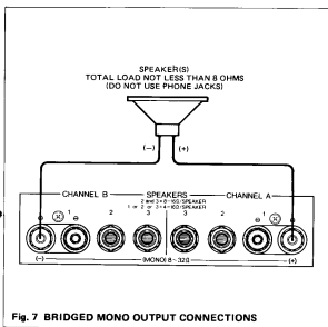
Fig. 7 BRIDGED MONO OUTPUT CONNECTIONS
