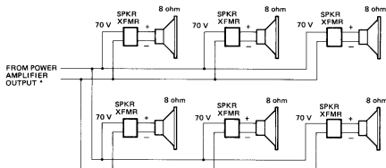
Fig. 19 A TYPICAL 70-VOLT DISTRIBUTED SYSTEM
