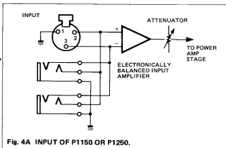
Fig. 4A INPUT OF P1150 OR P1250.
