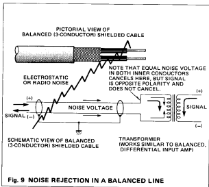
Fig. 9 NOISE REJECTION IN A BALANCED LINE
