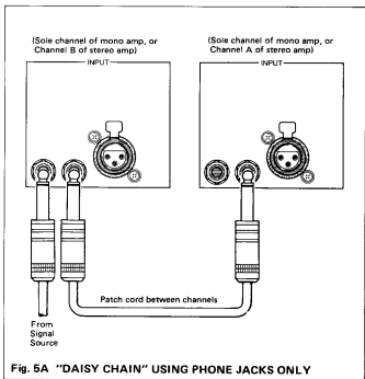
Fig. 5A "DAISY CHAIN" USING PHONE JACKS ONLY
