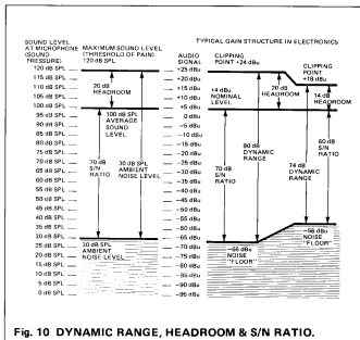
Fig. 10 DYNAMIC RANGE, HEADROOM & S/N RATIO.
