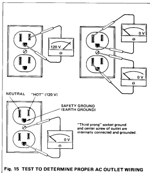
FIG. 15 TEST TO DETERMINE PROPER AC OUTLET WIRING
